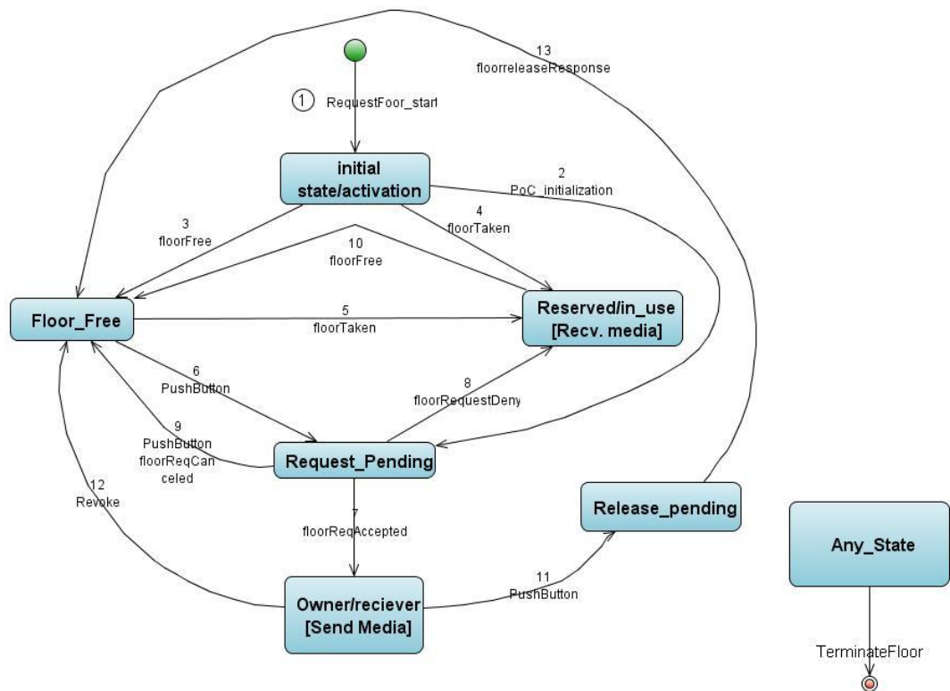
Figure 12: State diagram of the floor control.
