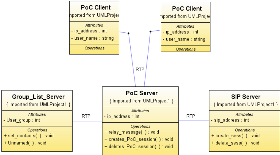
Figure 11: Class diagrams of the solution’s application domain.
