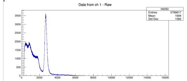
Figure 4.a: A energy spectrogram for the detector to the left of the radioactive source. (counts / channel)
