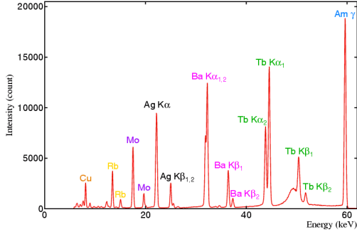
Figure 2: An Example Energy Spectrogram using a variety of radioactive sources [3]
