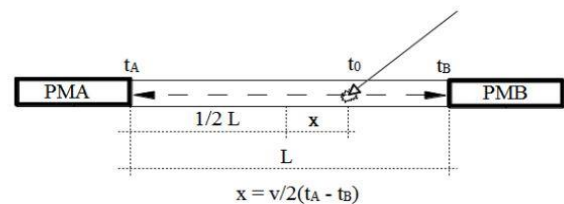
Figure 1: Diagram Depicting the calculation of the position of a radioactive point source in 1D space
